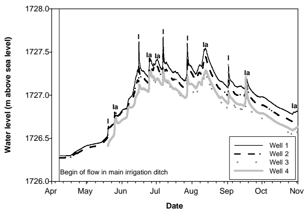
Figure 4. Well water level response to on-field irrigation (I) and nearby field irrigation (Ia) during the 2005 irrigation season.
