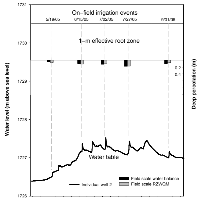
Figure 5. Shallow groundwater response to calculated (water balance method) and simulated (RZWQM) deep percolation in well 2 after five on-field irrigations during the 2005 season.
