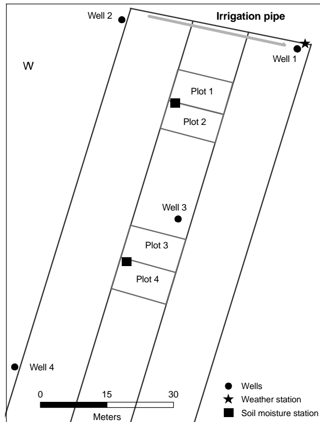
Figure 1. Layout of the deep percolation study site at the Alcalde Science Center.
