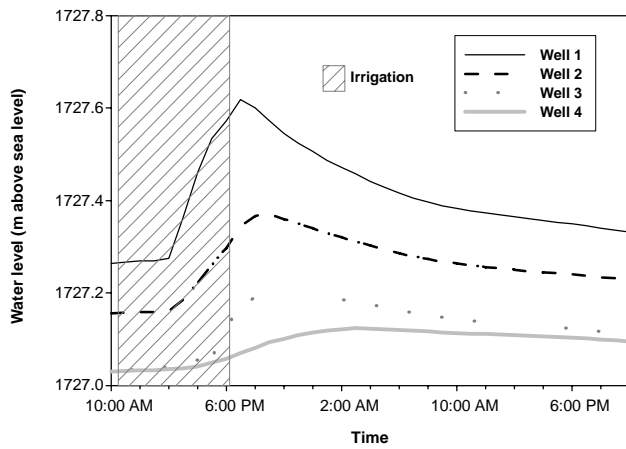
Figure 3. Water level fluctuations in four experimental wells in response to the irrigation event of 15 June 2005.
