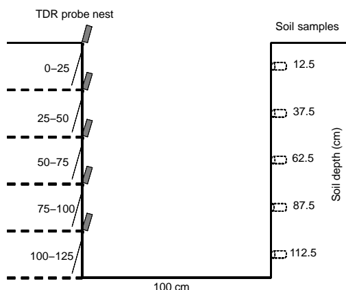
Figure 2. Schematic of TDR probe nest installation and bulk soil sample collection in one excavated pit.
